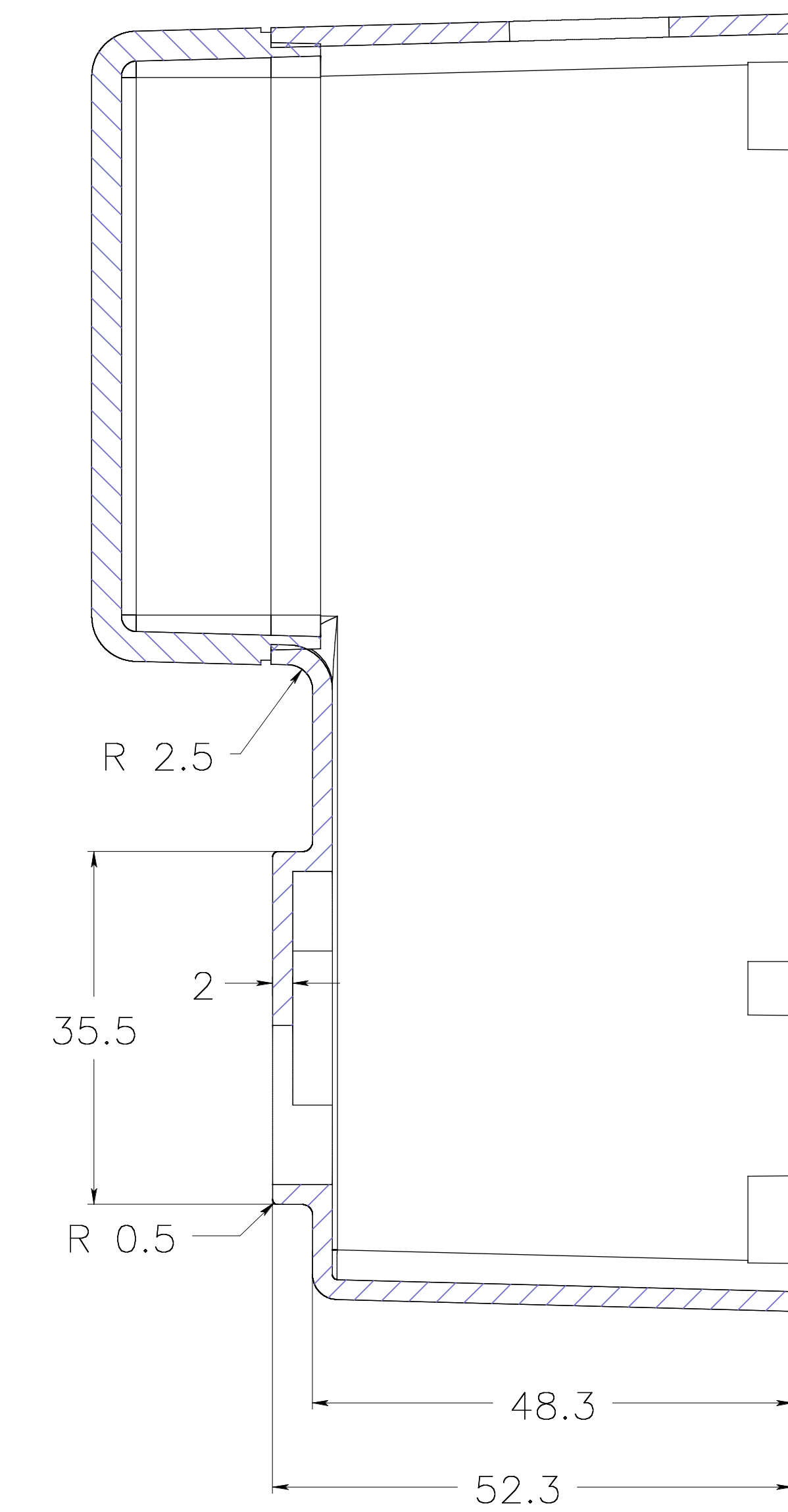
section AA
