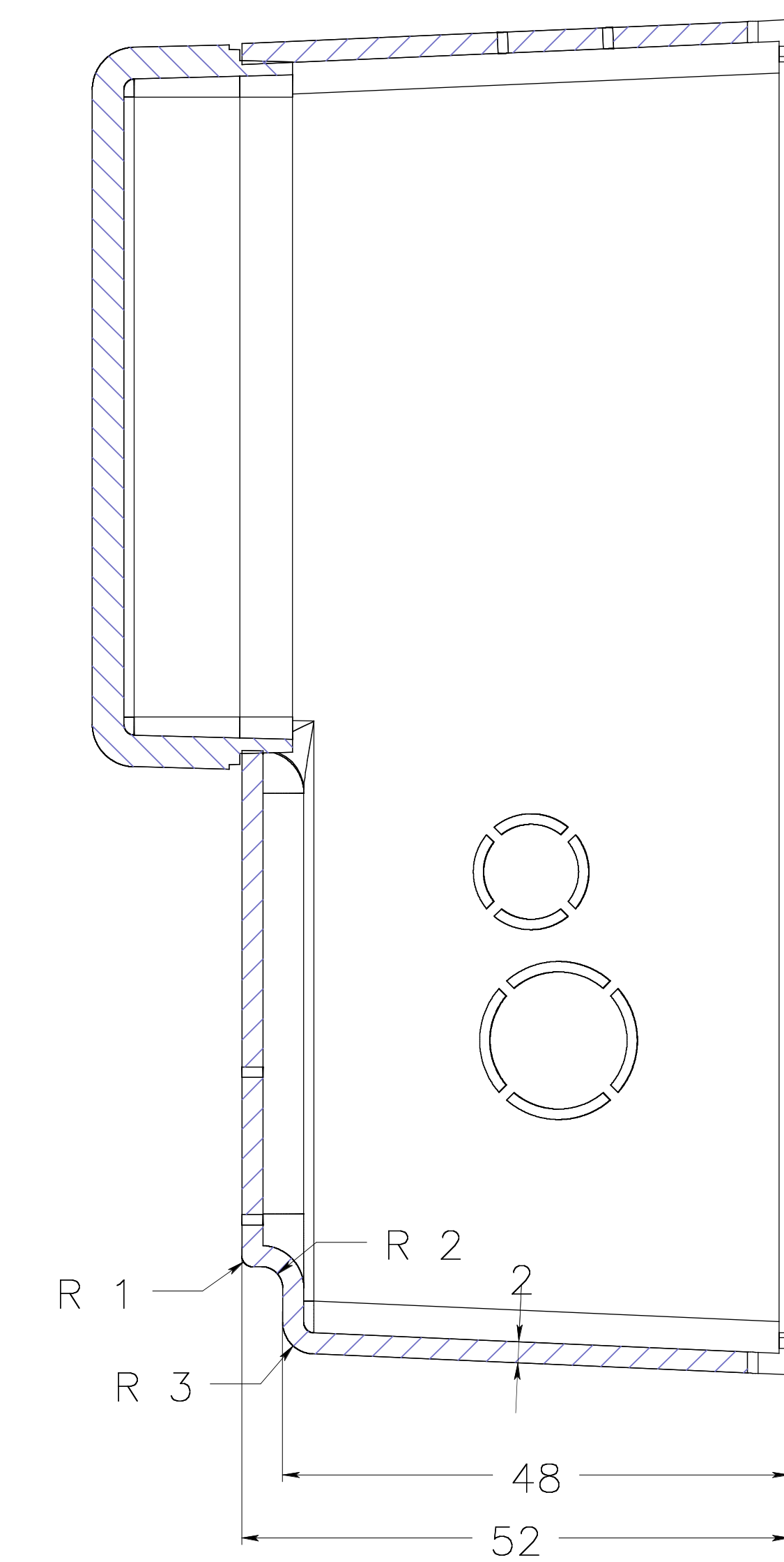
section AA
