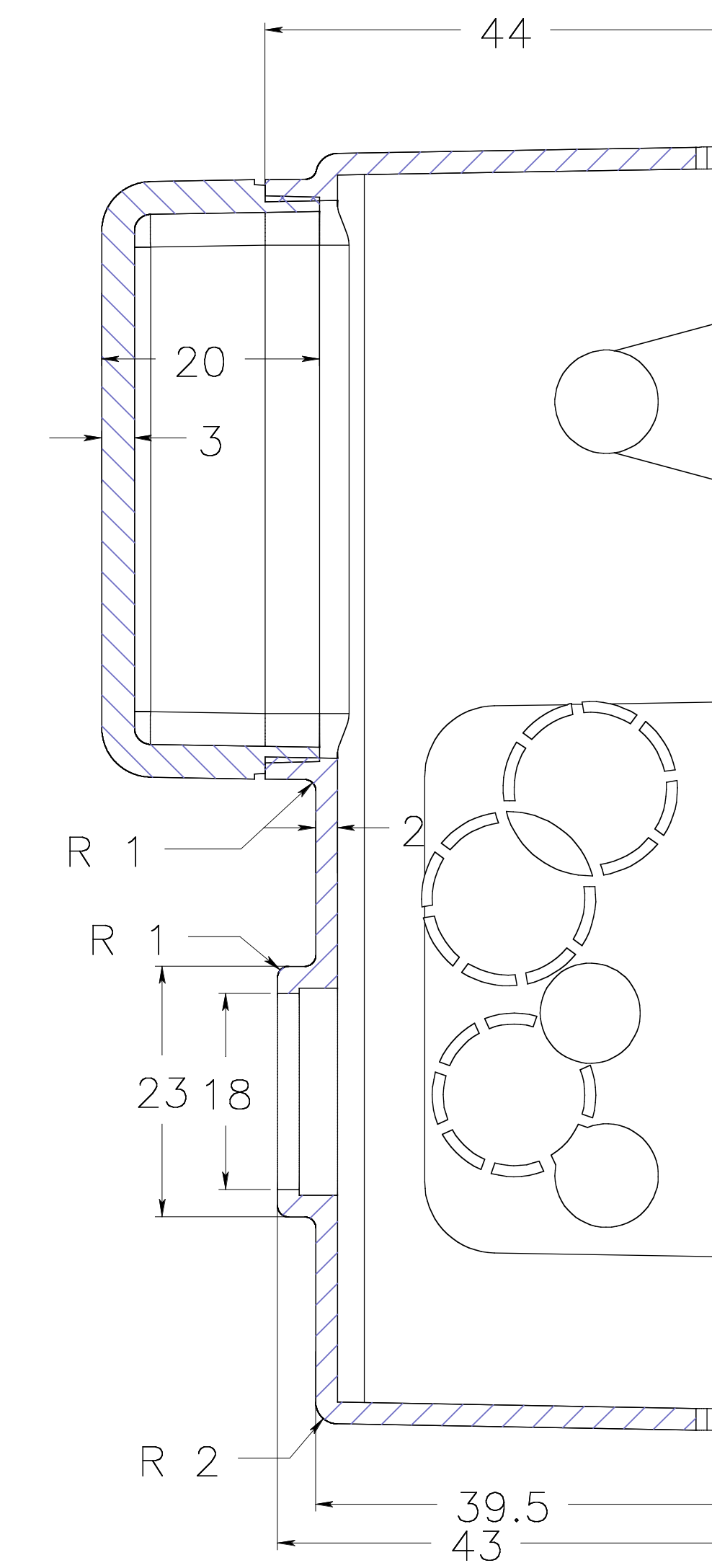
section BB
