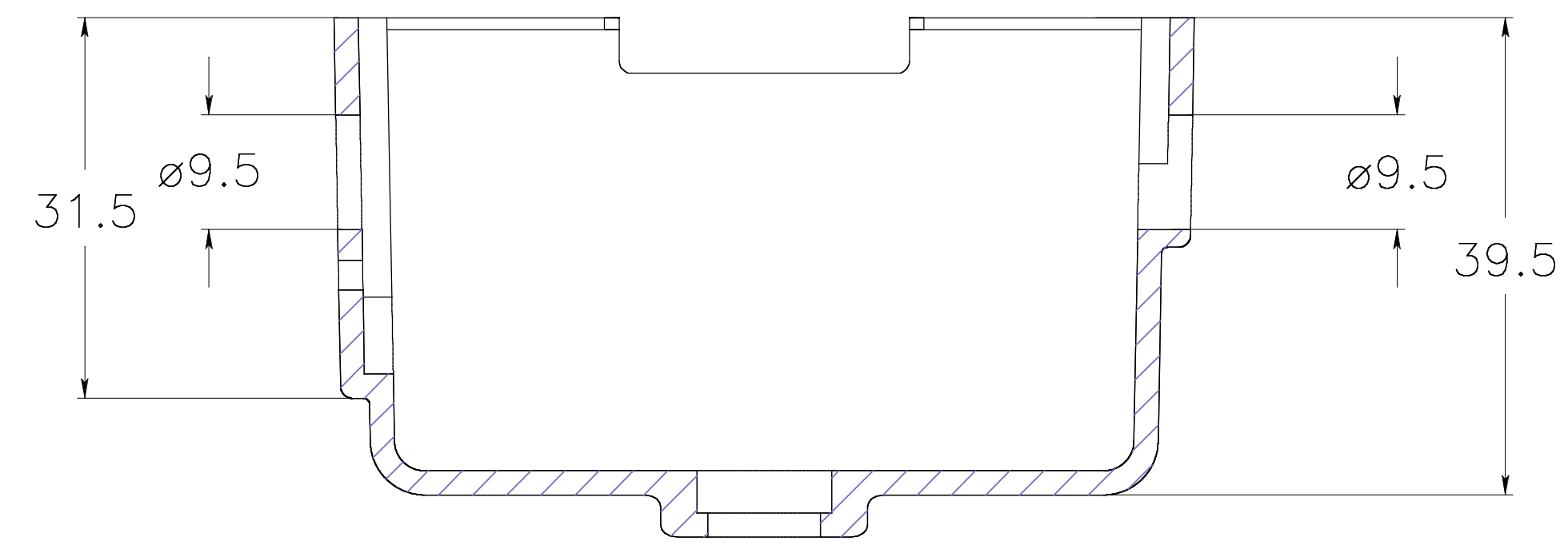
section AA
