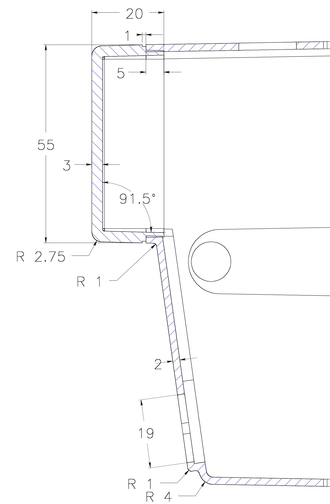
section BB
