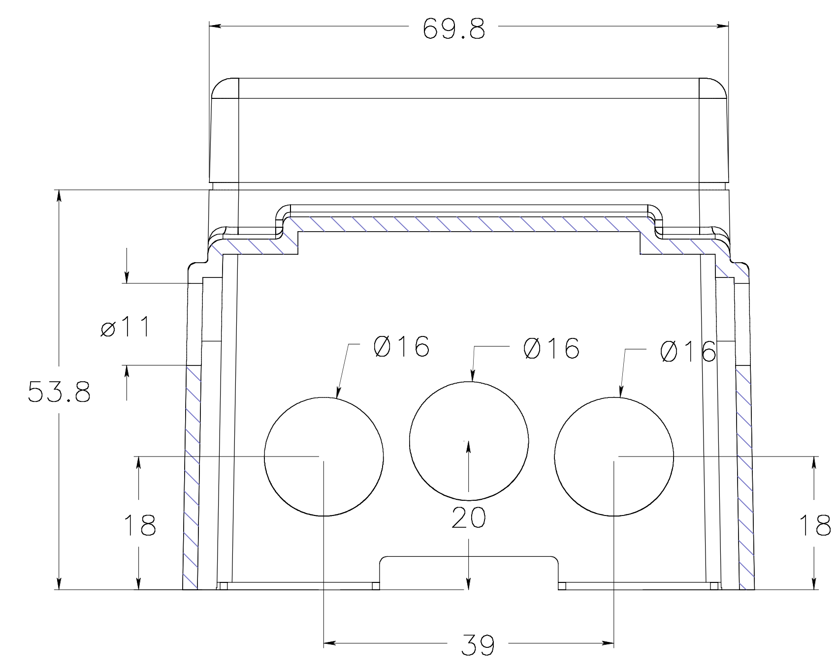
section AA
