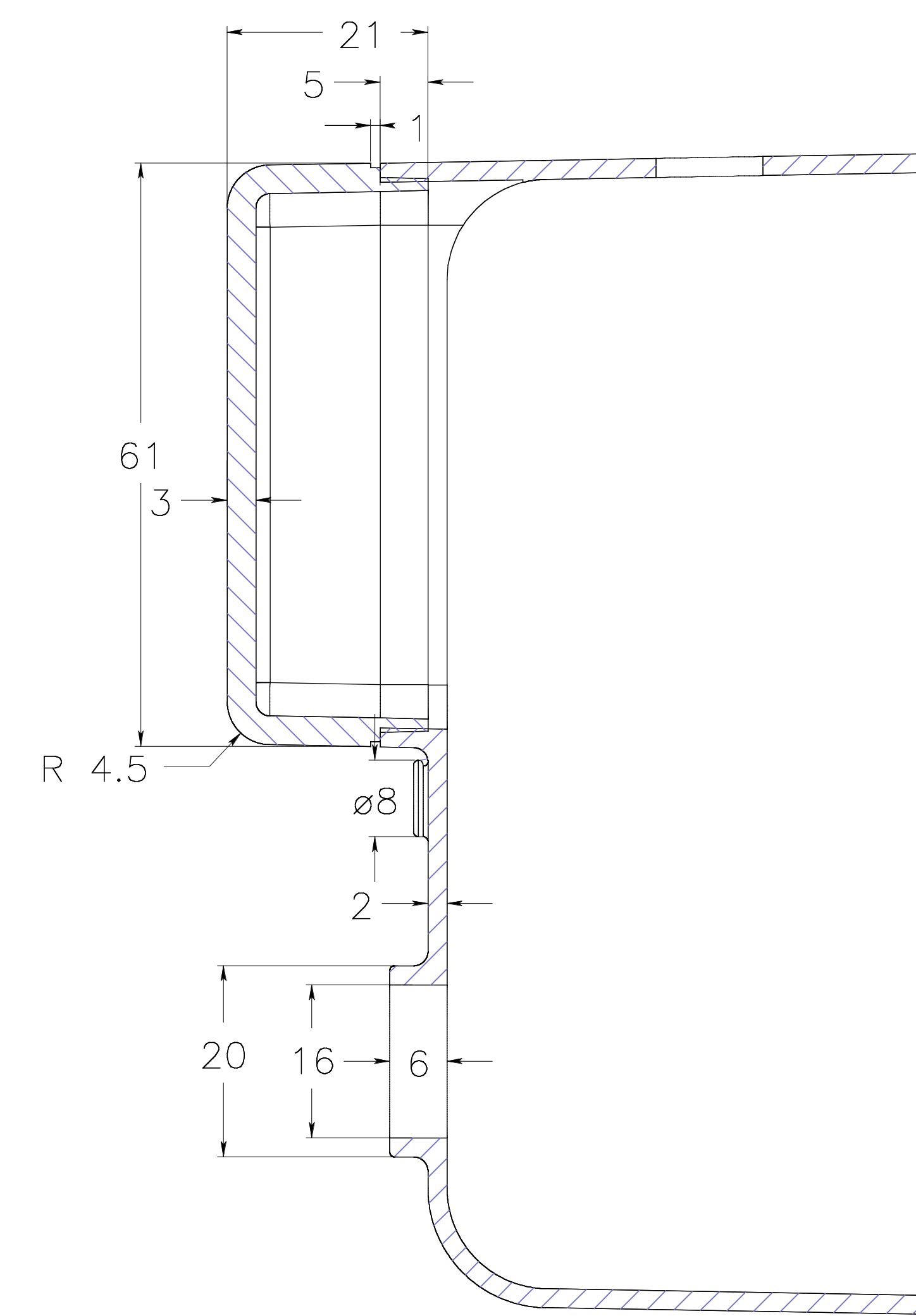
section AA
