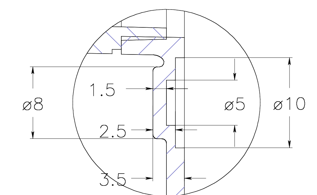
detail C
