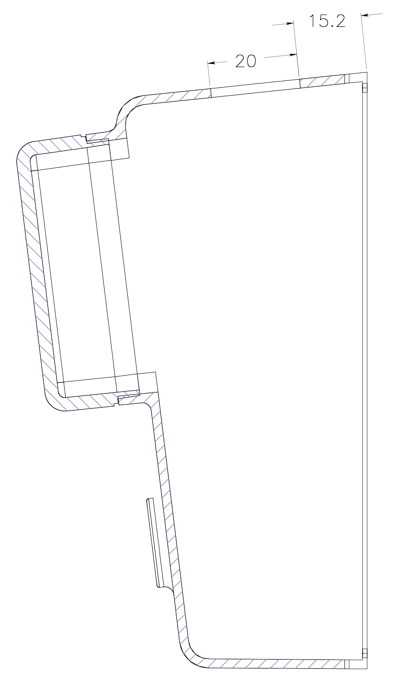
section BB
