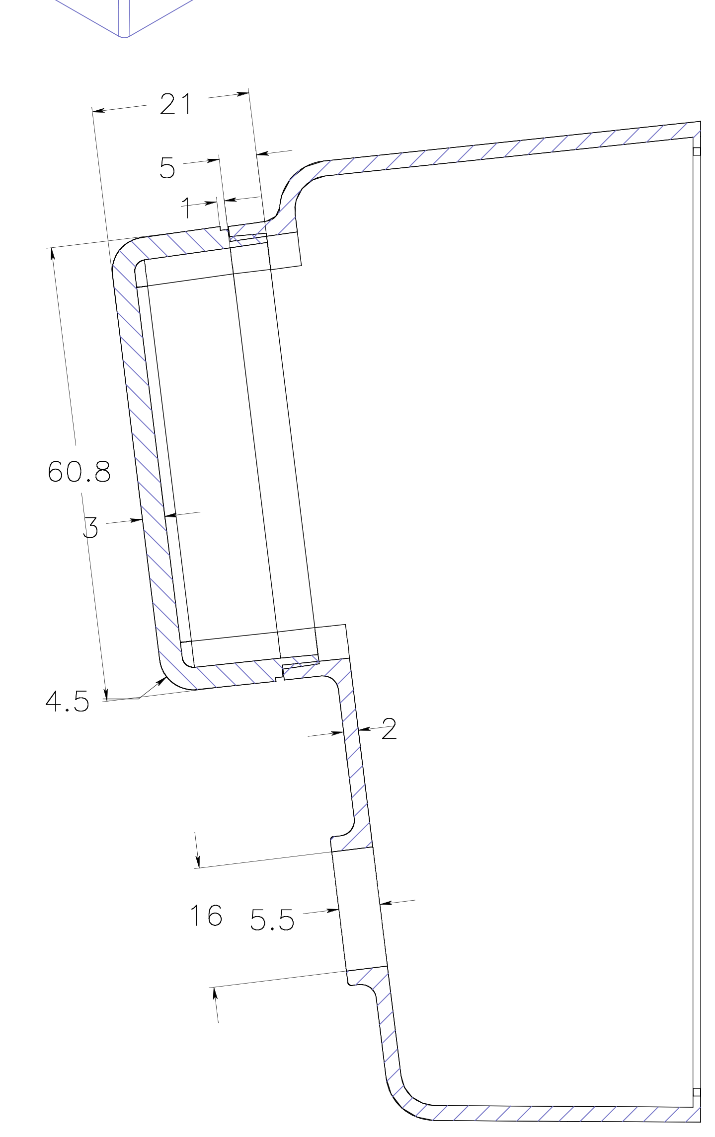
section AA
