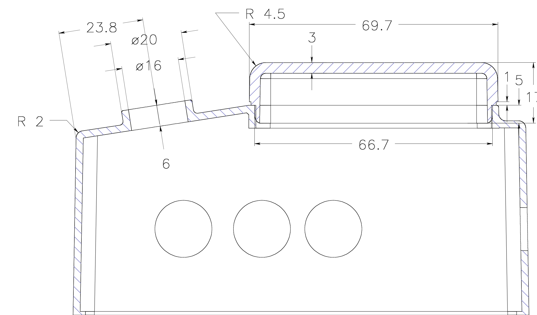
section AA
