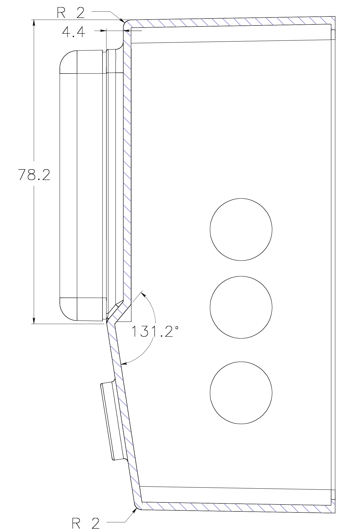
section BB
