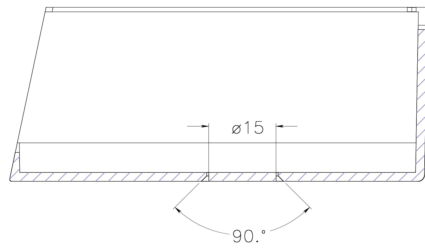
section FF
