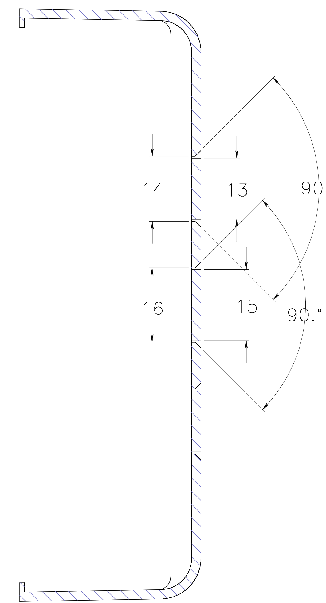
section EE
