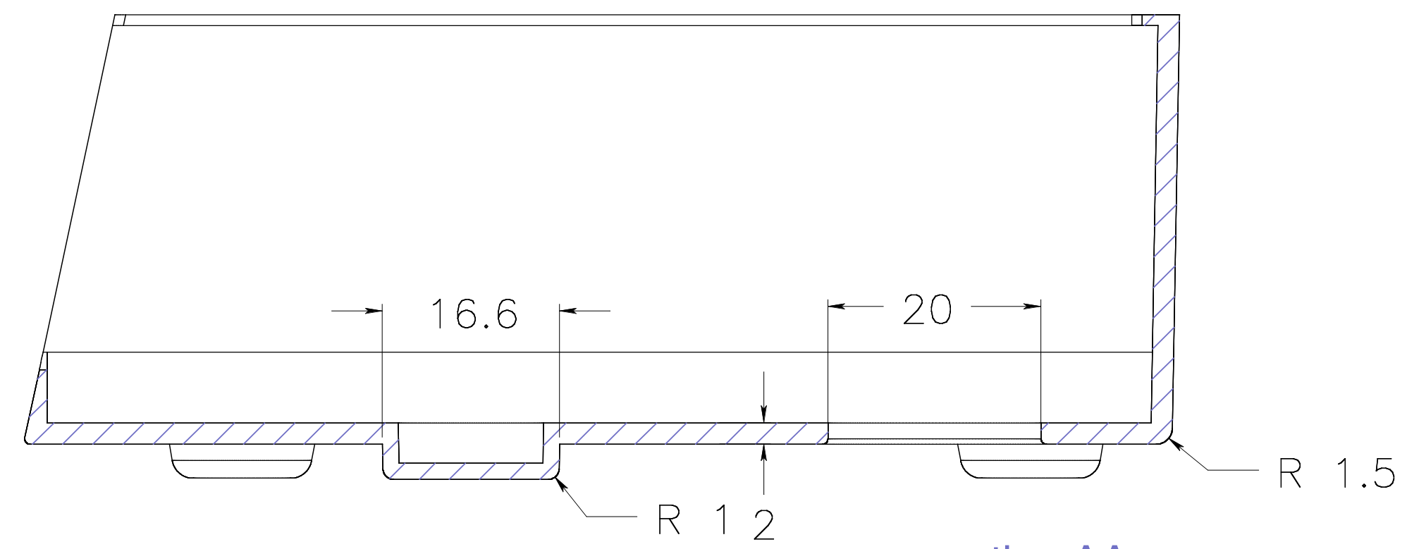
section AA
