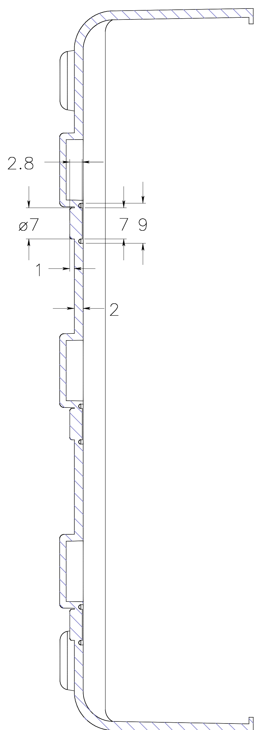
section BB
