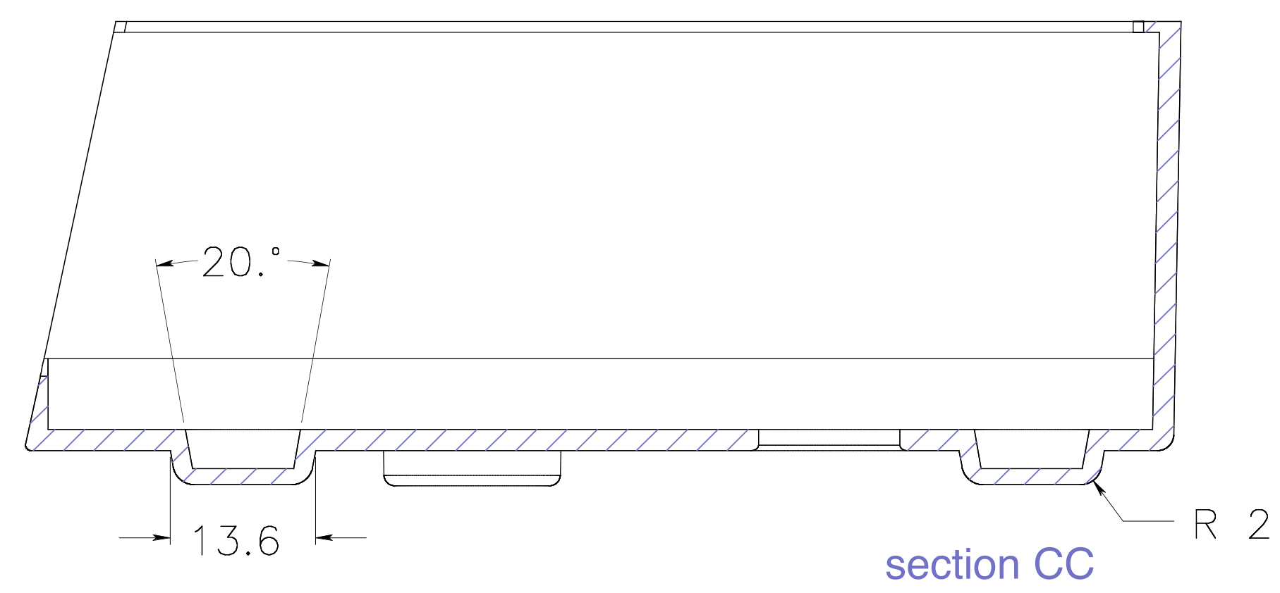
section CC
