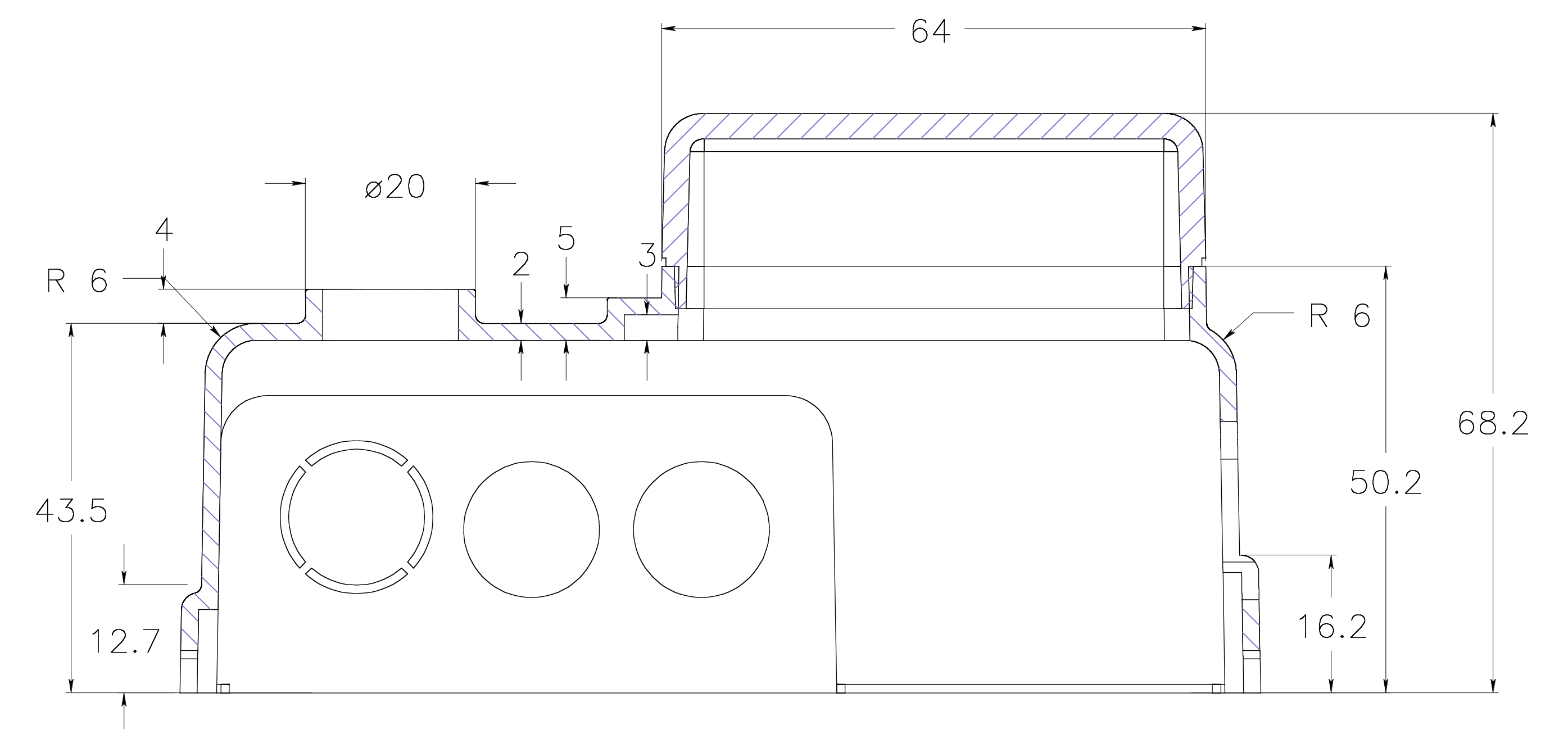
section FF
